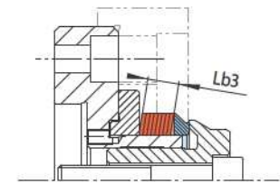
Bonded disc pack width Lb3
