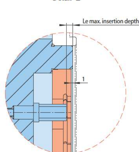
Detail "Z"
