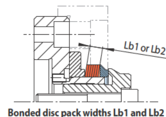
Bonded disc pack widths Lb1 and Lb2
